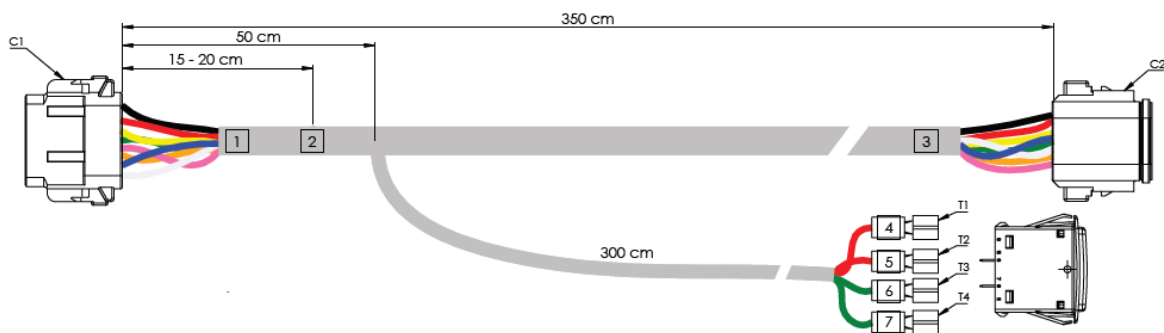
New Track Controller harness
